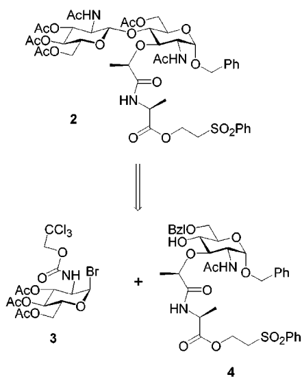
Scheme 1. Retrosynthetic Analysis of the Lipid II Glycopeptide Core
